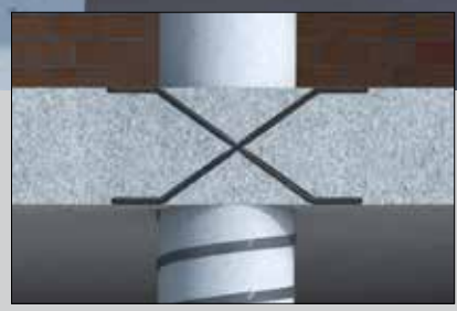
SikaWrap® FX to strengthen beam-column joints
